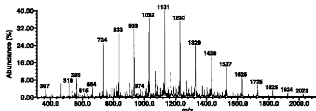
Figure 3. Electrospray MS analysis of product produced from DMA polymerization by initiator 3 in 9:1 H_2O :dioxane using ligand 4 ; theoretical M_n = 2000 g/mol.
