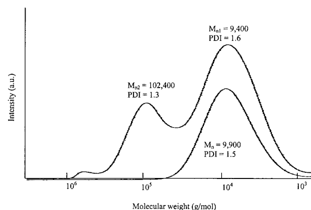
Figure 1. Gel permeation chromatography analysis of PDMA in sequential monomer addition experiment. Monomodal distribution corresponds to the first monomer addition, theoretical M_n = 2500 g/mol, and the bimodal distribution was obtained after the second monomer addition, theoretical M_n = 5000 g/mol.
