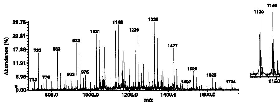
Figure 2. Electrospray MS analysis of product produced from DMA polymerization by initiator 1 in 9:1 toluene:DMF using ligand 6 ; theoretical M_n = 2500 g/mol.
